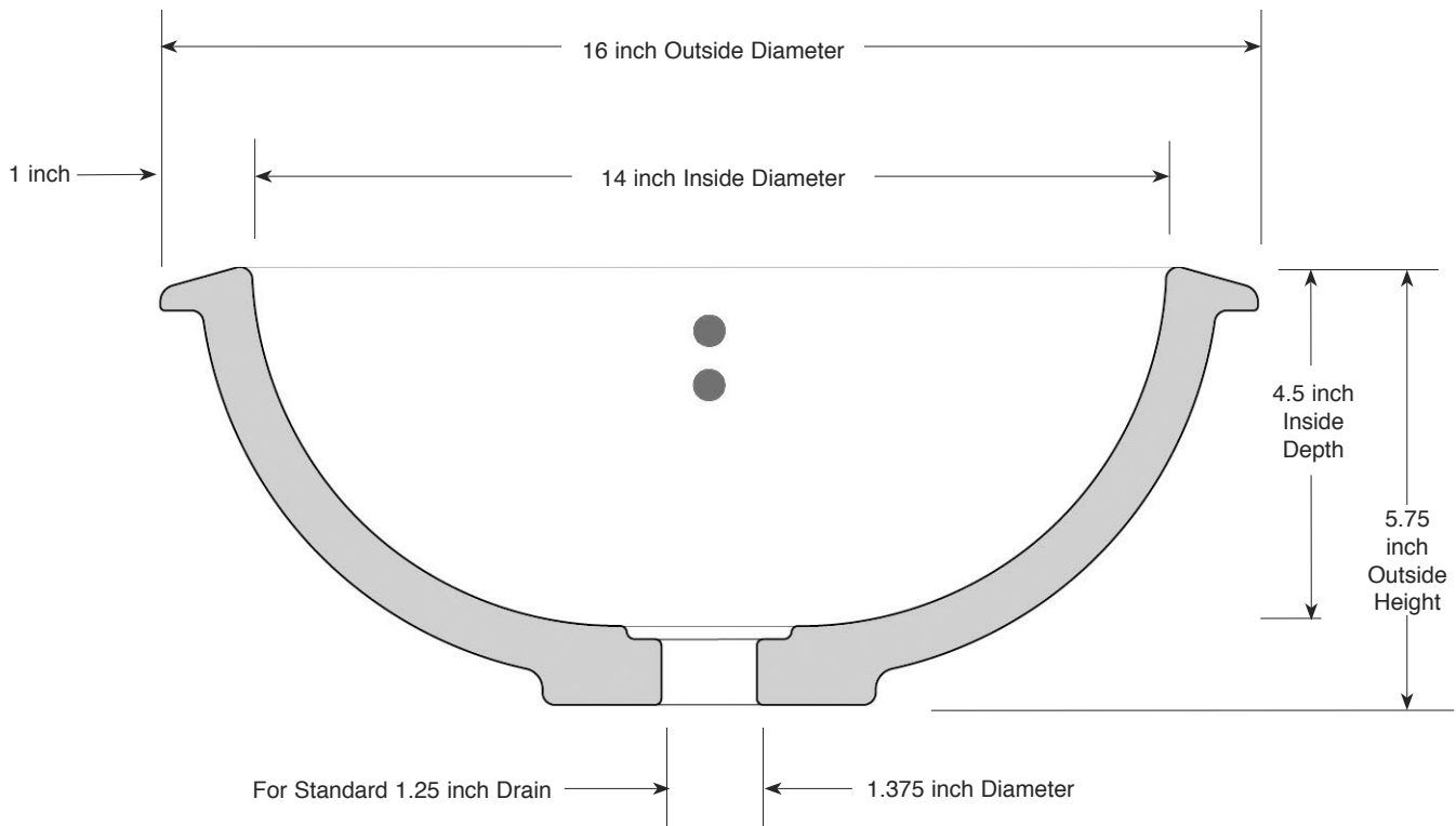
Standard 16 Inch Rimmed Basin – Not To Scale
